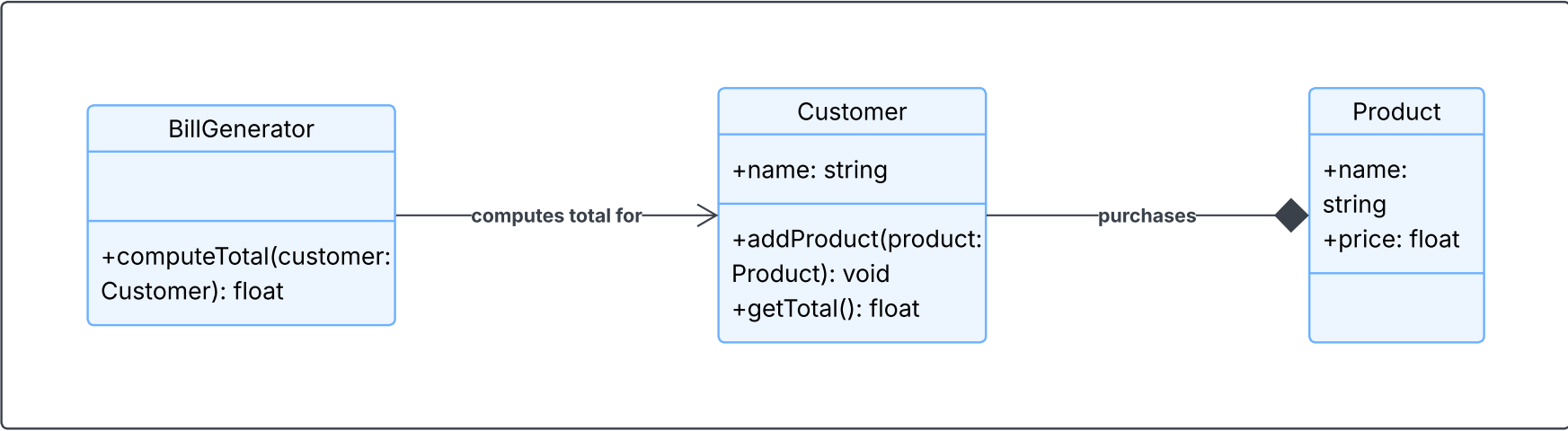
Grocery Store Bill Generation Application - Class Diagram
