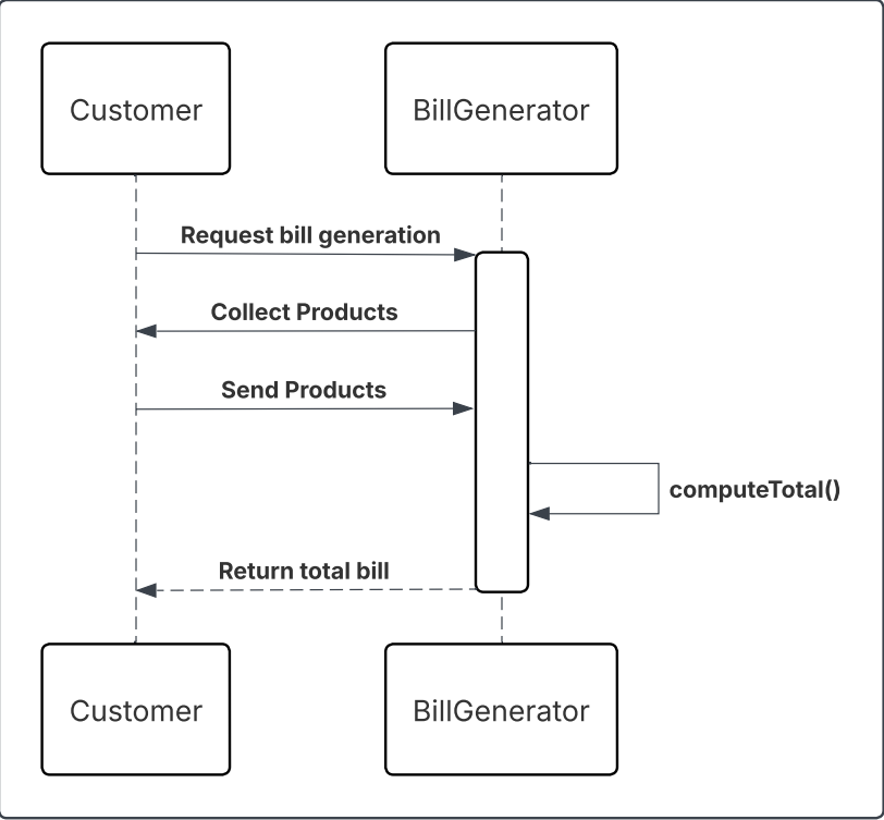
Sequence Diagram for Grocery Store Bill Generation
